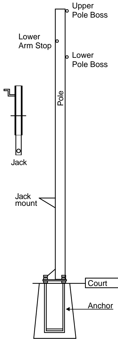
(Side View)
